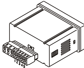
EXCITATION VOLTAGE SELECTION: 24 V or 10 V
