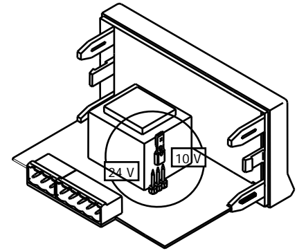
EXCITATION VOLTAGE SELECTION: 24 V or 10 V
